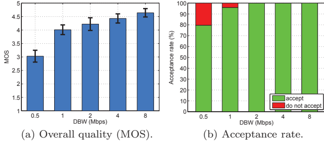
Figure 4: QoE in Facebook Mobile.
