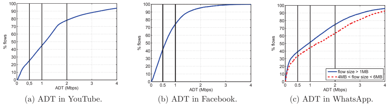
Figure 8: Flow ADT in a cellular network for YouTube, Facebook and WhatsApp.
