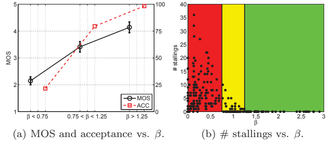
Figure 2: \beta = ADT/VBR as a QoE-related KPI.
