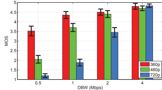
Figure 3: QoE in YouTube – smartphones.
