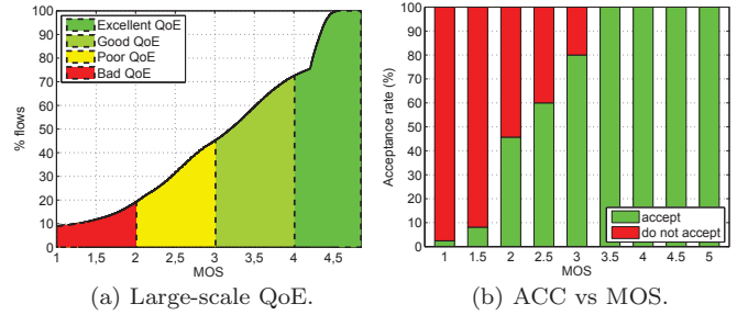
Figure 7: DBW-QoE modeling & evaluation.
