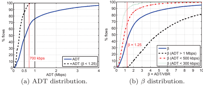
Figure 6: YouTube QoE in a fixed-line network.
