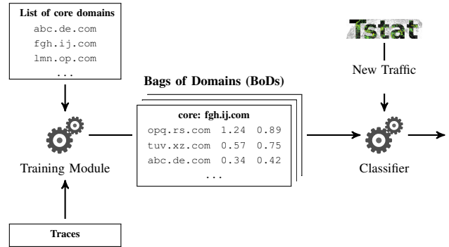
Figure 2: WHAT architecture.
